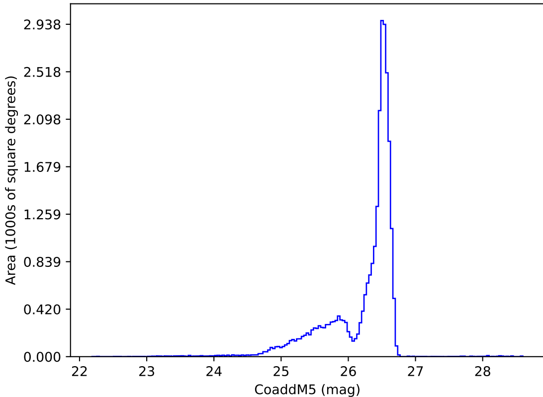
ddf_acor_sf10_lsf40_lsr10_v3.4_10yrs i: CoaddM5
