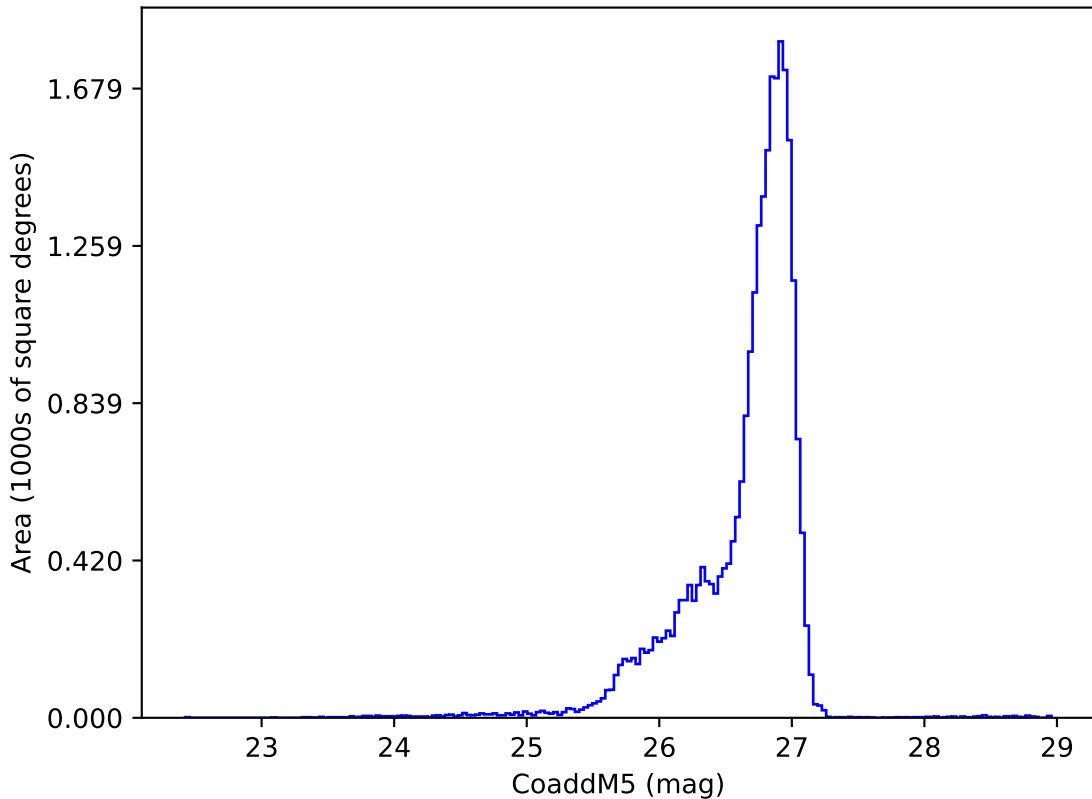
ddf_acor_sf10_lsf40_lsr10_v3.4_10yrs g: CoaddM5
