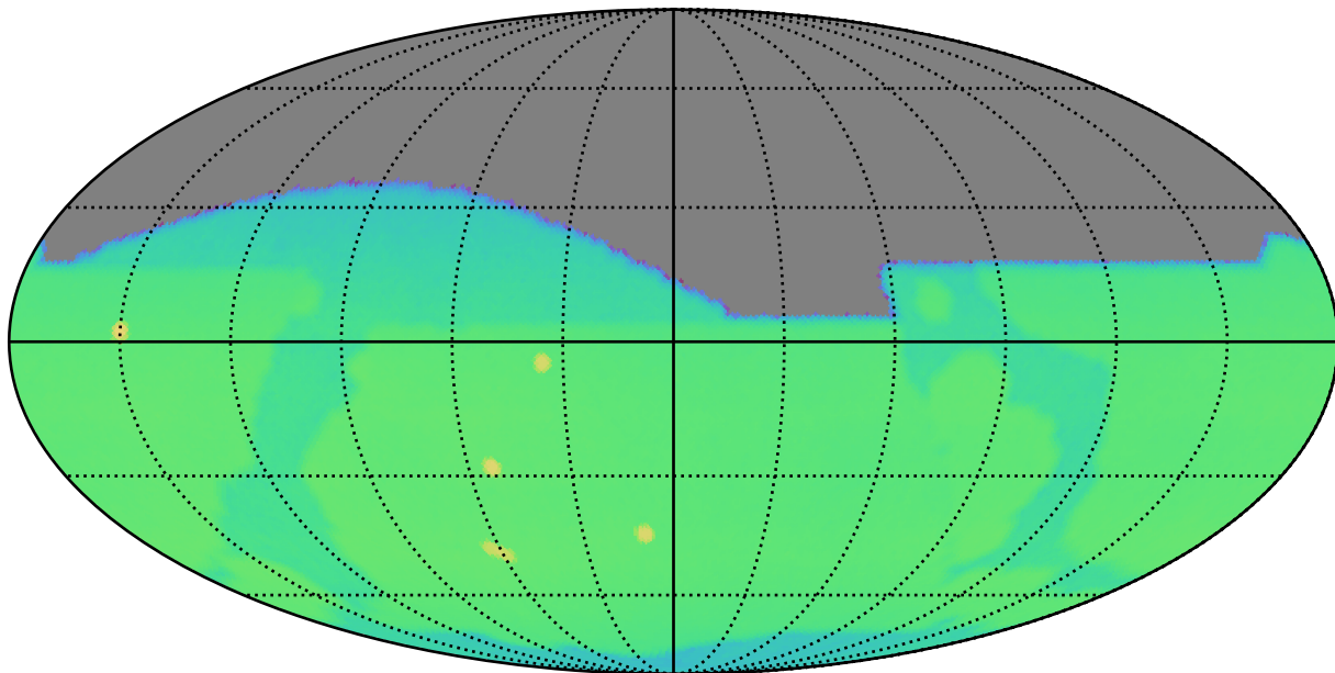
ddf_acor_sf10_lsf40_lsr10_v3.4_10yrs : CoaddM5
