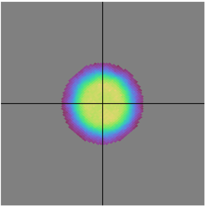
ddf_acor_sf10_lsf40_lsr10_v3.4_10yrs all bands: DD:COSMOS N Unique Nights
