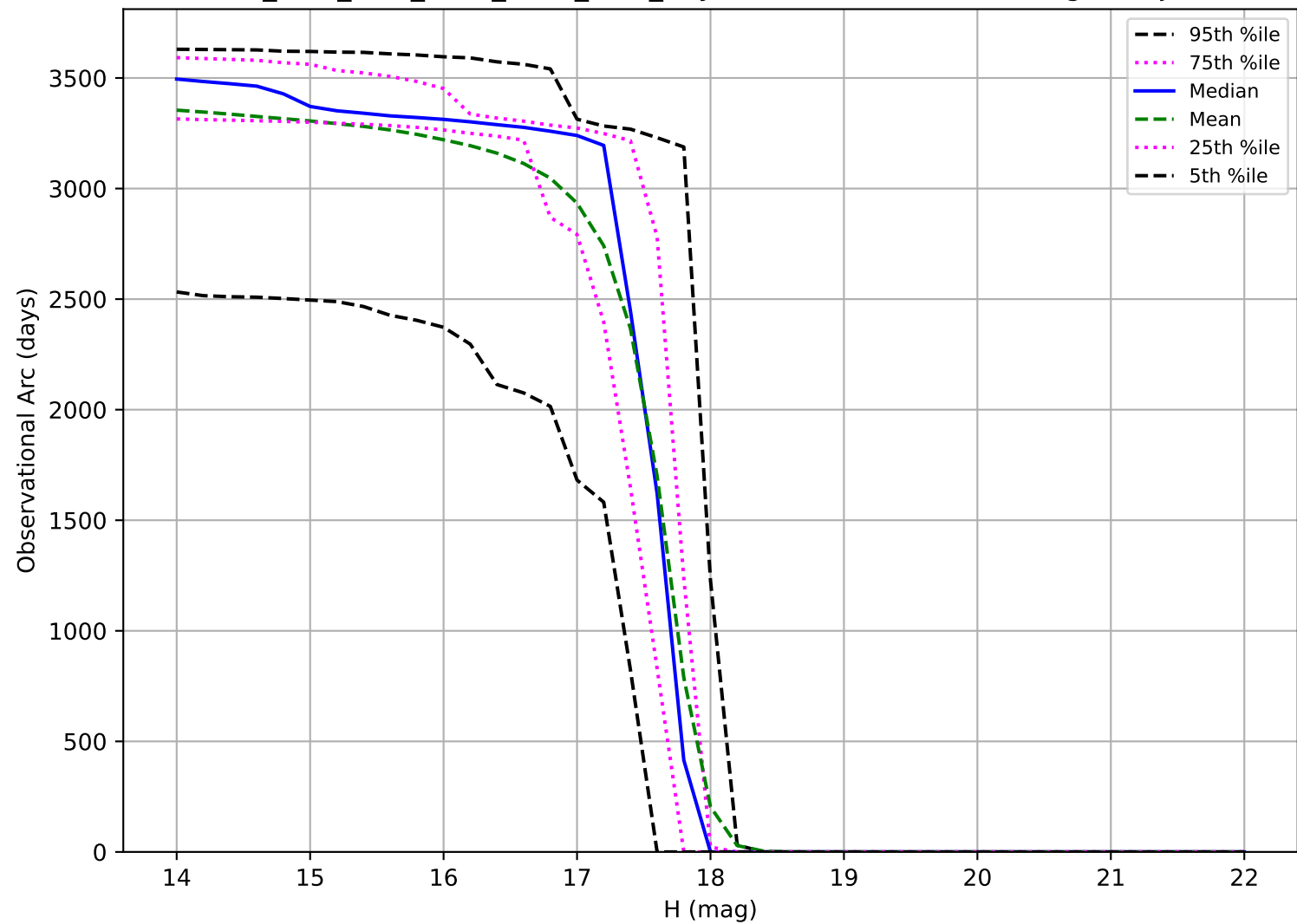
ddf_acor_sf10_lsf30_lsr50_v3.4_10yrs: Observational Arc Length Trojan
