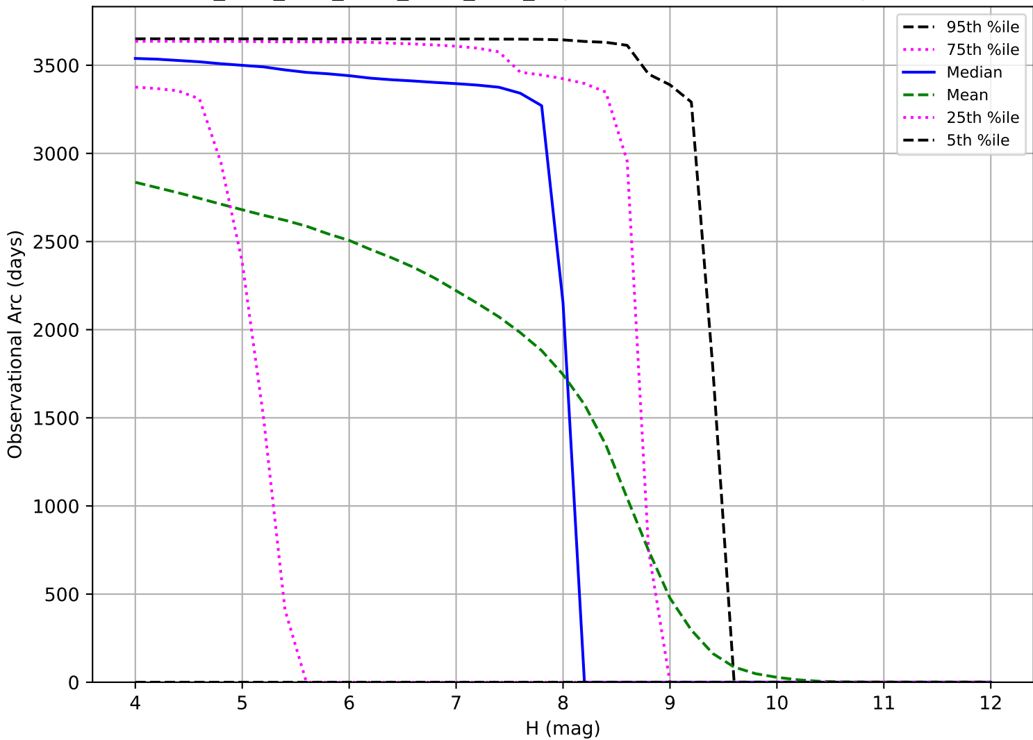
ddf_acor_sf10_Isf30_Isr50_v3.4_10yrs: Observational Arc Length TNO
