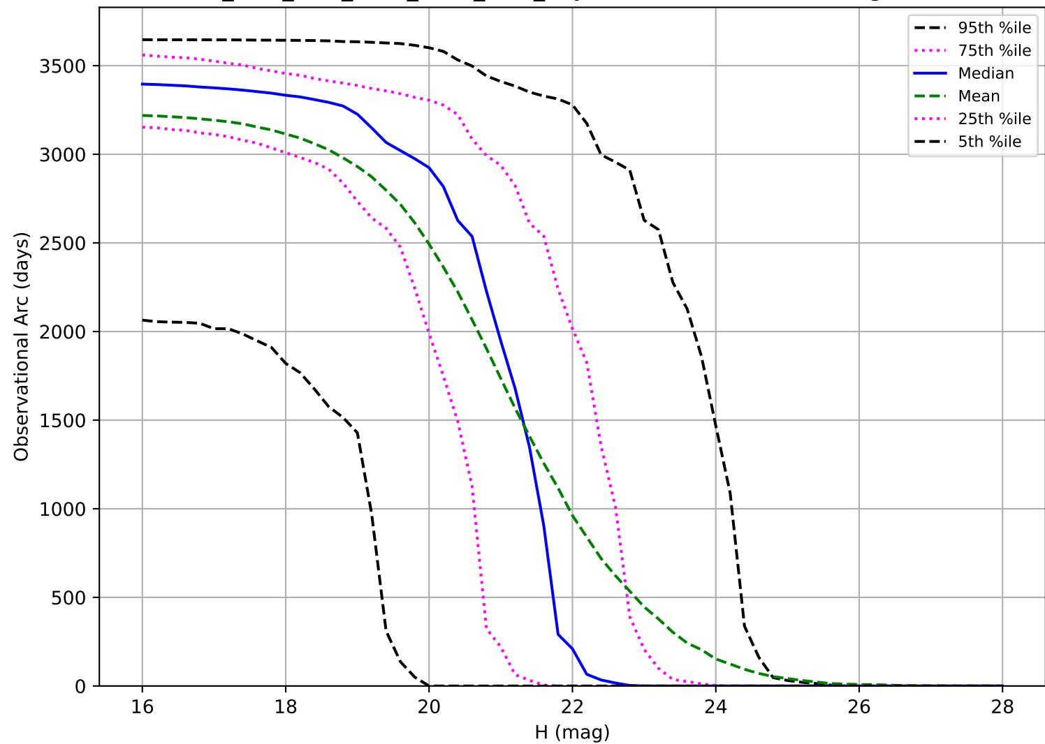
ddf_acor_sf10_lsf30_lsr50_v3.4_10yrs: Observational Arc Length PHA
