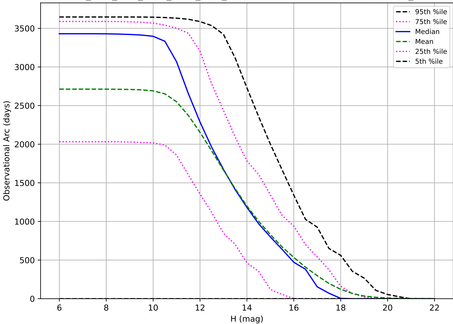
ddf_acor_sf10_lsf30_lsr50_v3.4_10yrs: Observational Arc Length OCC_r5
