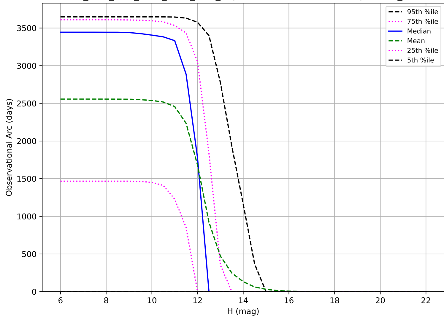
ddf_acor_sf10_lsf30_lsr50_v3.4_10yrs: Observational Arc Length OCC_r20
