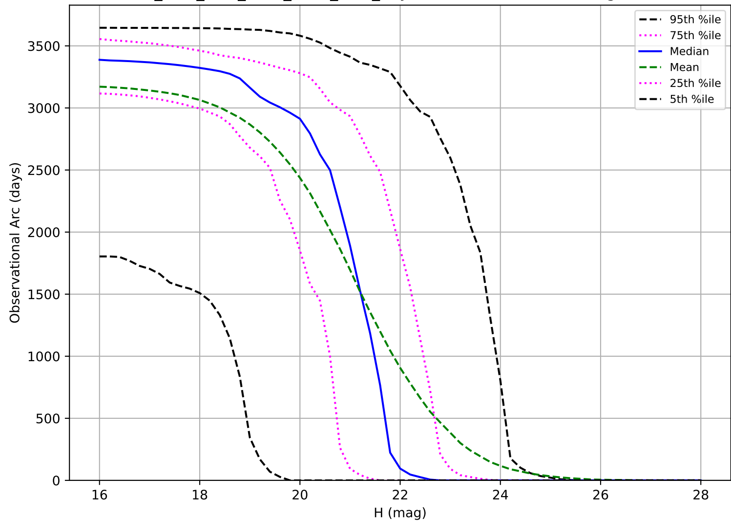
ddf_acor_sf10_lsf30_lsr50_v3.4_10yrs: Observational Arc Length NEO
