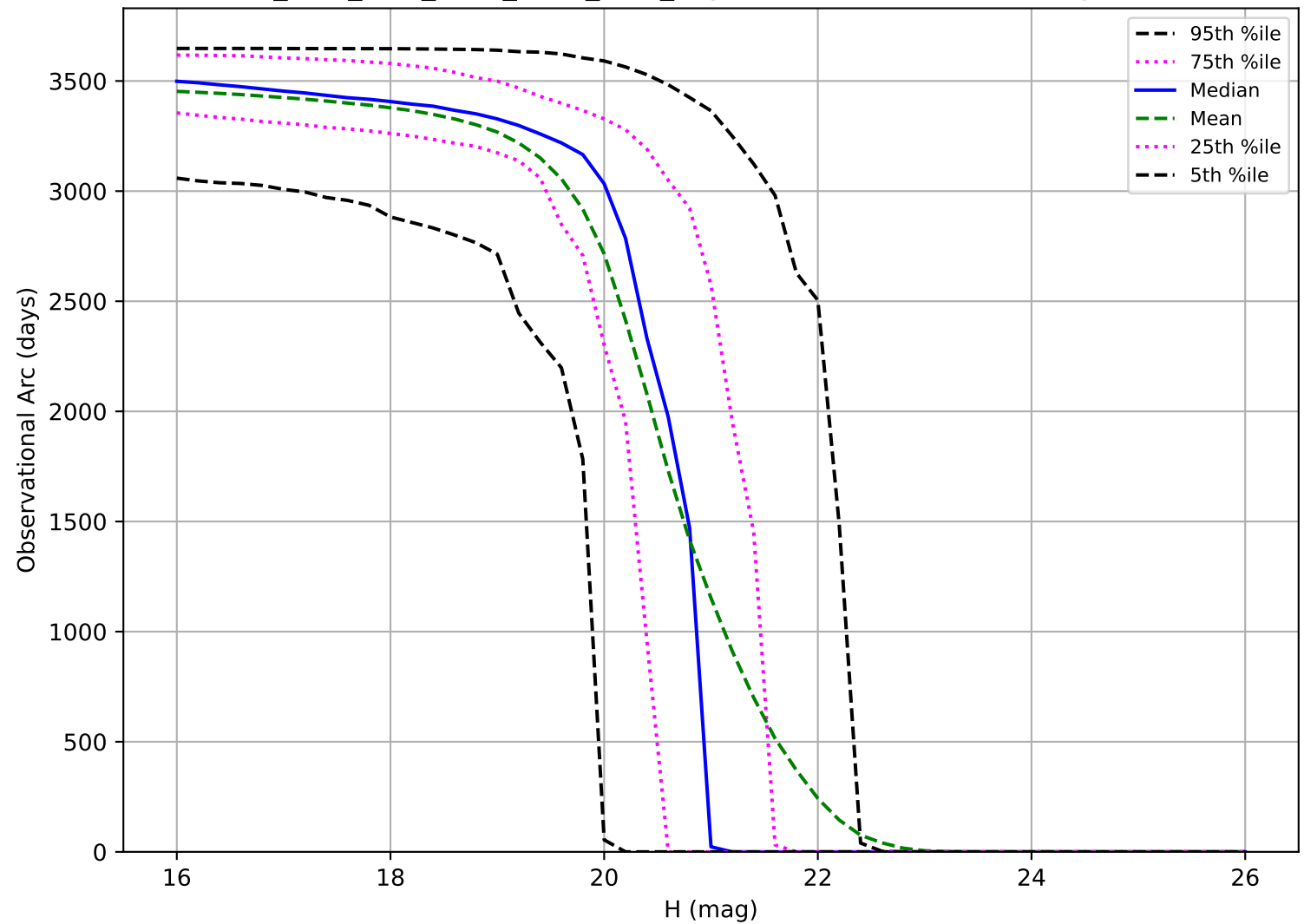
ddf_acor_sf10_lsf30_lsr50_v3.4_10yrs: Observational Arc Length MBA
