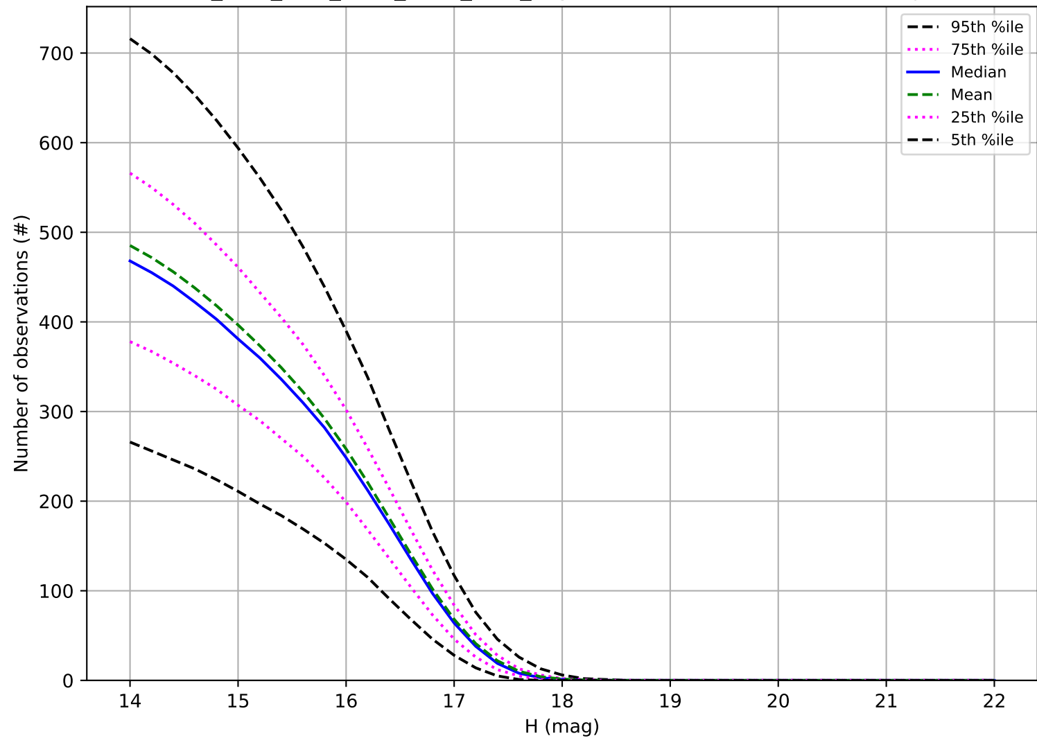
ddf_acor_sf10_lsf30_lsr50_v3.4_10yrs: Number of observations Trojan
