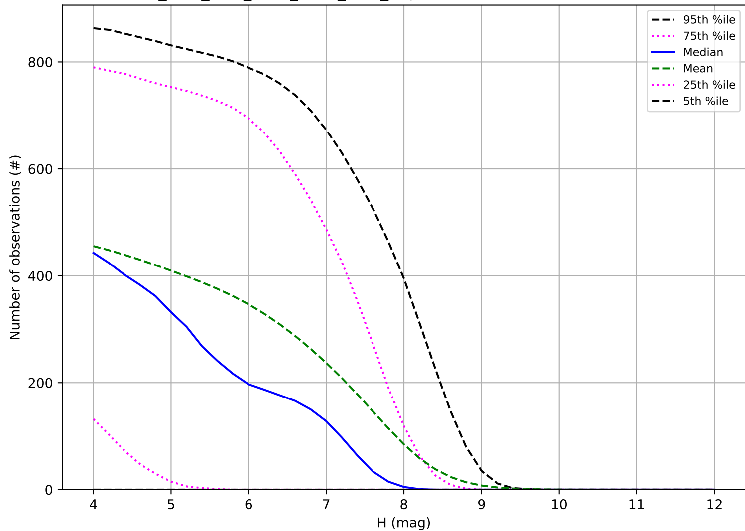
ddf_acor_sf10_lsf30_lsr50_v3.4_10yrs: Number of observations TNO
