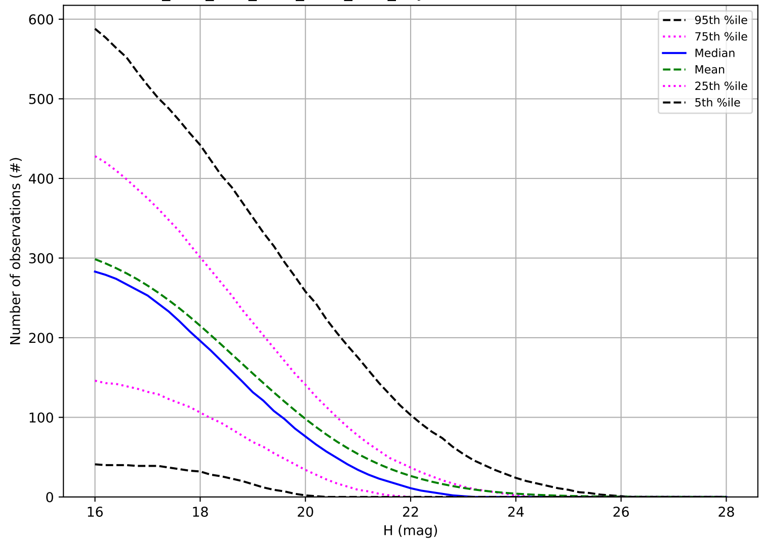
ddf_acor_sf10_lsf30_lsr50_v3.4_10yrs: Number of observations PHA
