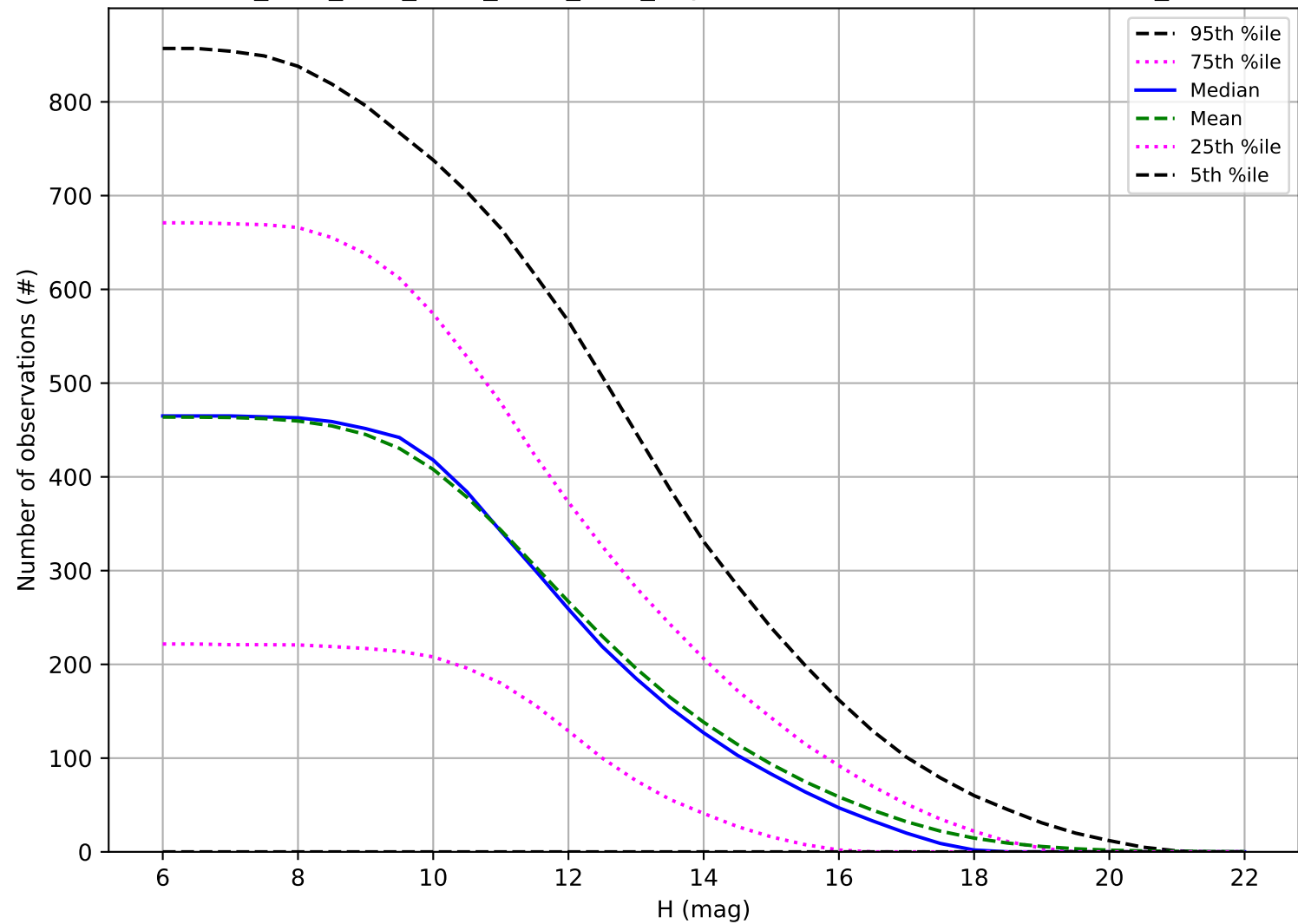
ddf_acor_sf10_lsf30_lsr50_v3.4_10yrs: Number of observations OCC_r5
