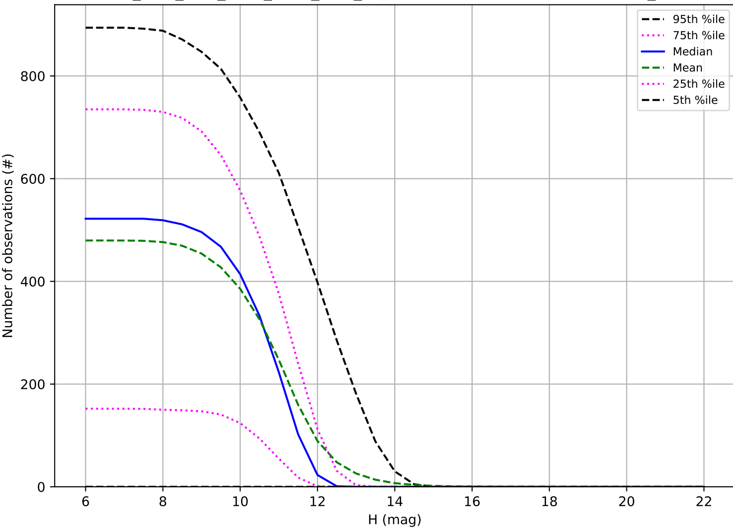
ddf_acor_sf10_lsf30_lsr50_v3.4_10yrs: Number of observations OCC_r20
