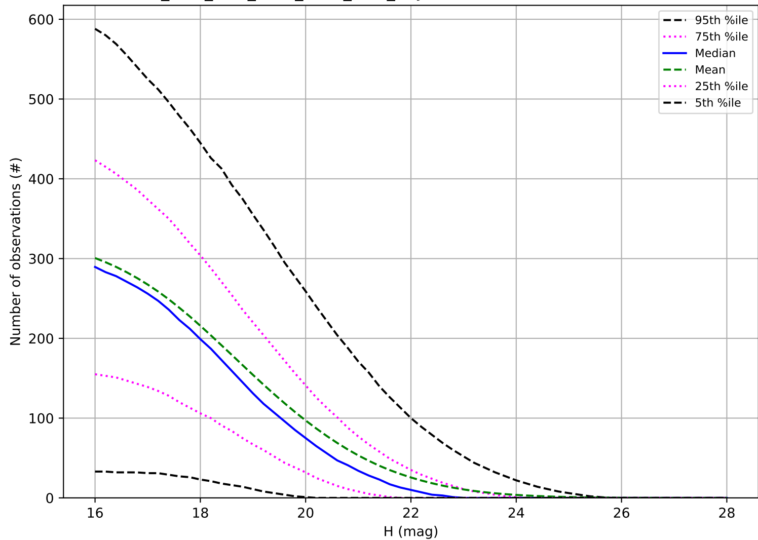
ddf_acor_sf10_lsf30_lsr50_v3.4_10yrs: Number of observations NEO
