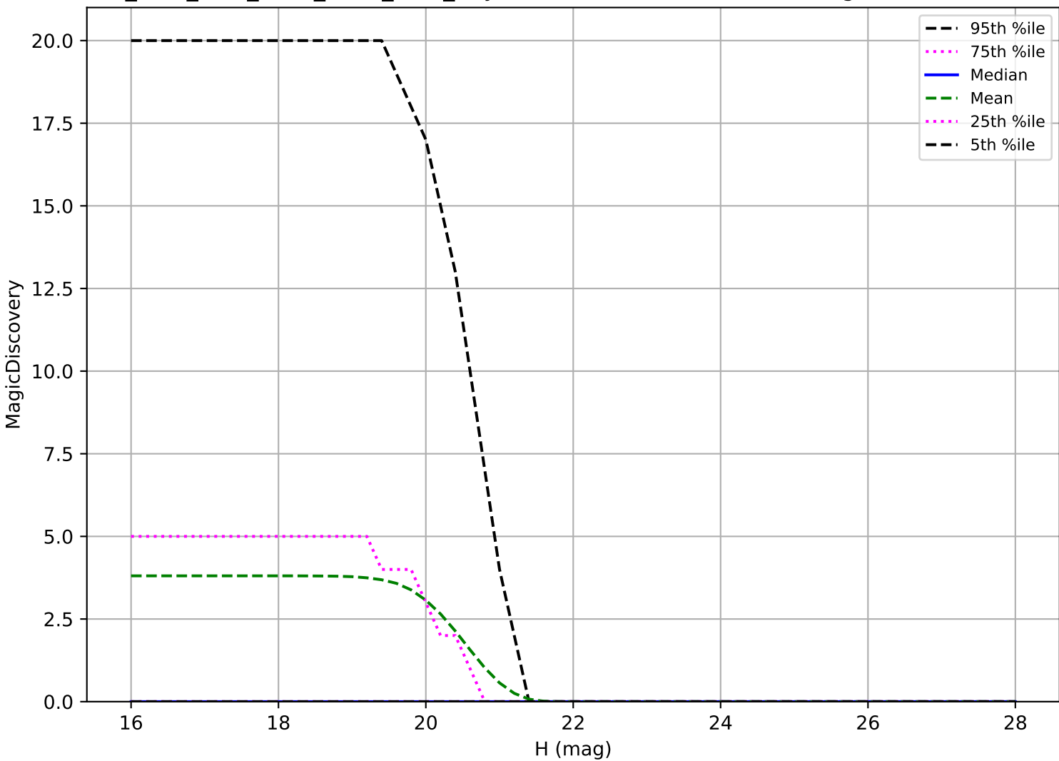
ddf_acor_sf10_lsf30_lsr50_v3.4_10yrs: Vatra 6 detections in 60 nights detection loss
