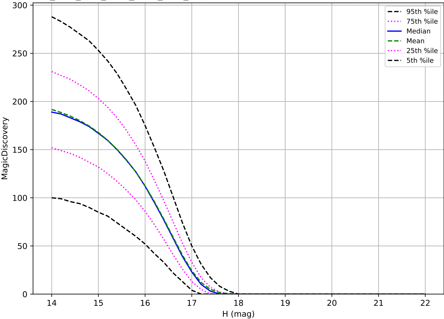
ddf_acor_sf10_lsf30_lsr50_v3.4_10yrs: Trojan 6 detections in 60 nights detection loss
