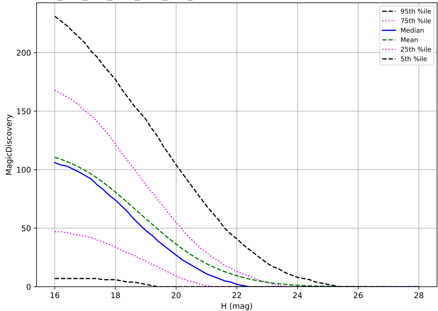
ddf_acor_sf10_lsf30_lsr50_v3.4_10yrs: PHA 6 detections in 60 nights detection loss
