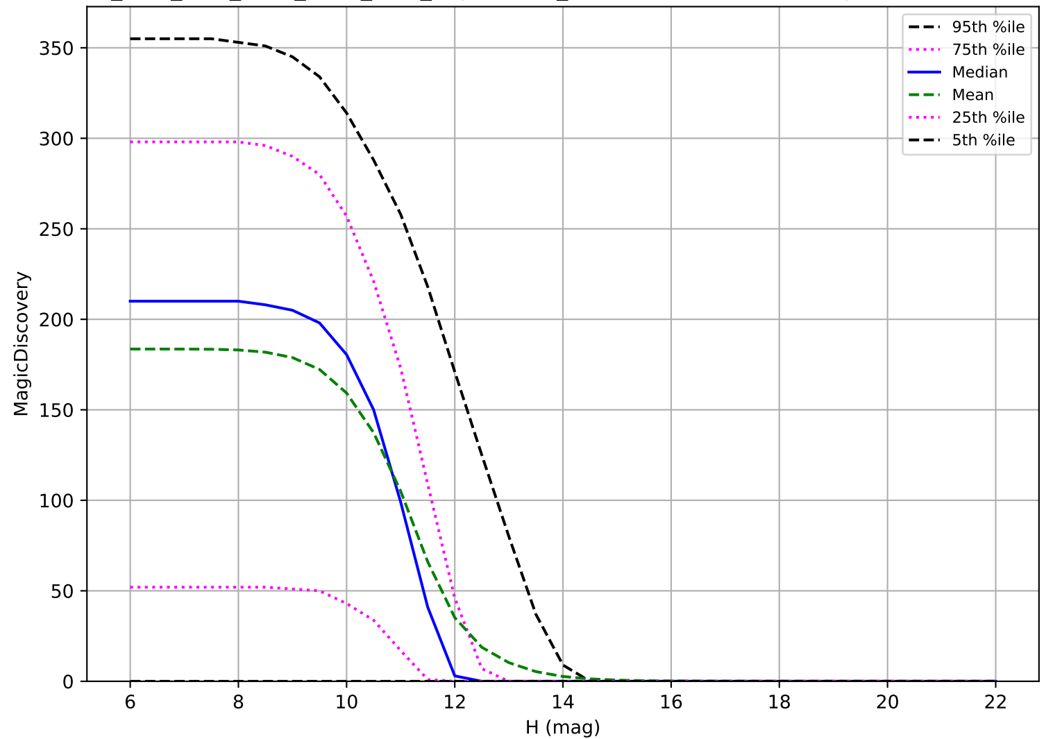
ddf_acor_sf10_lsf30_lsr50_v3.4_10yrs: OCC_r20 6 detections in 60 nights detection loss
