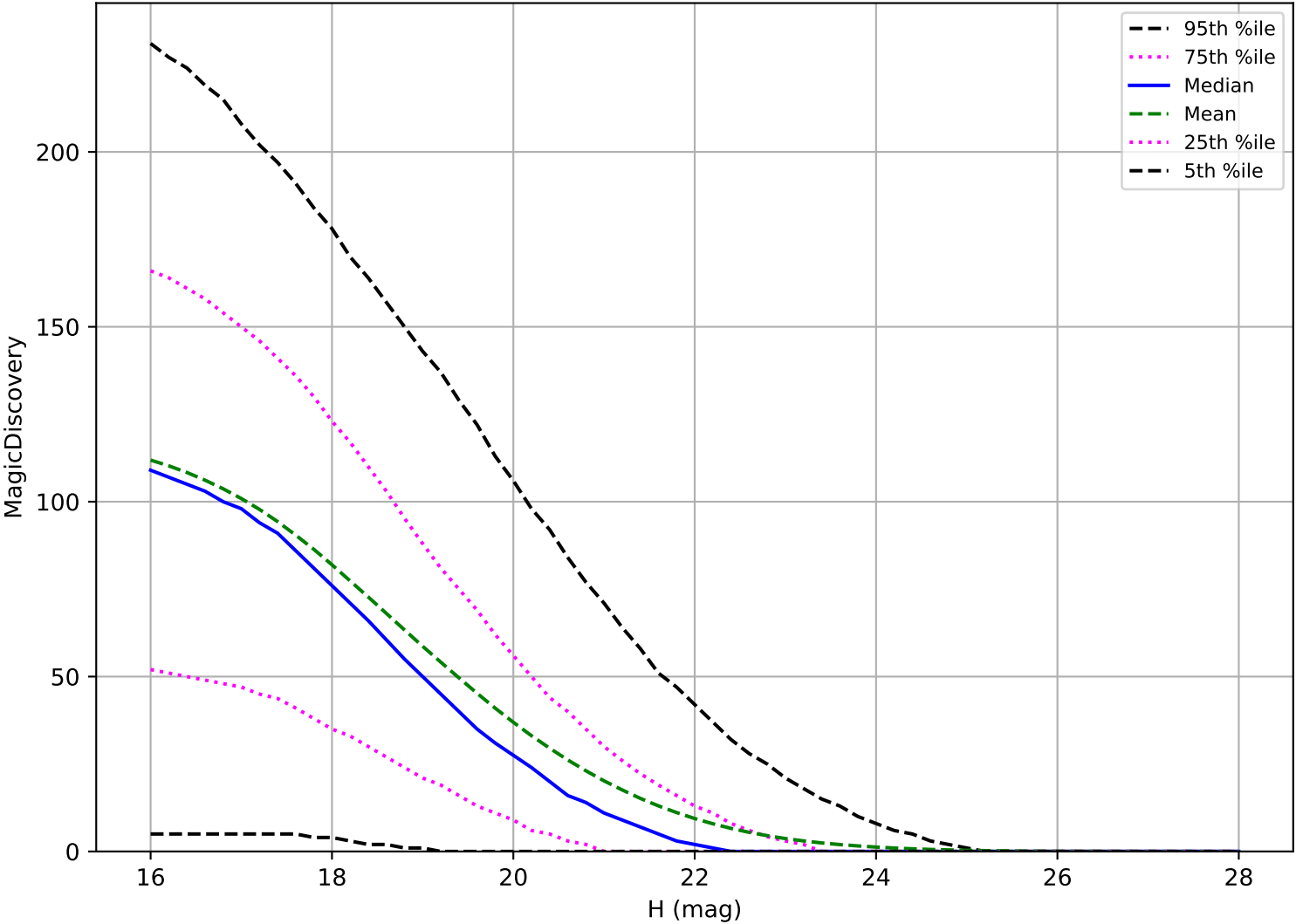
ddf_acor_sf10_lsf30_lsr50_v3.4_10yrs: NEO 6 detections in 60 nights detection loss
