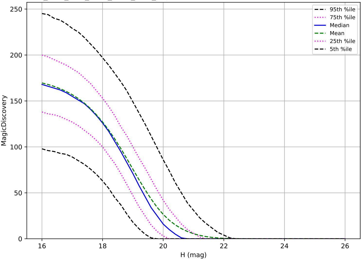
ddf_acor_sf10_lsf30_lsr50_v3.4_10yrs: MBA 6 detections in 60 nights detection loss
