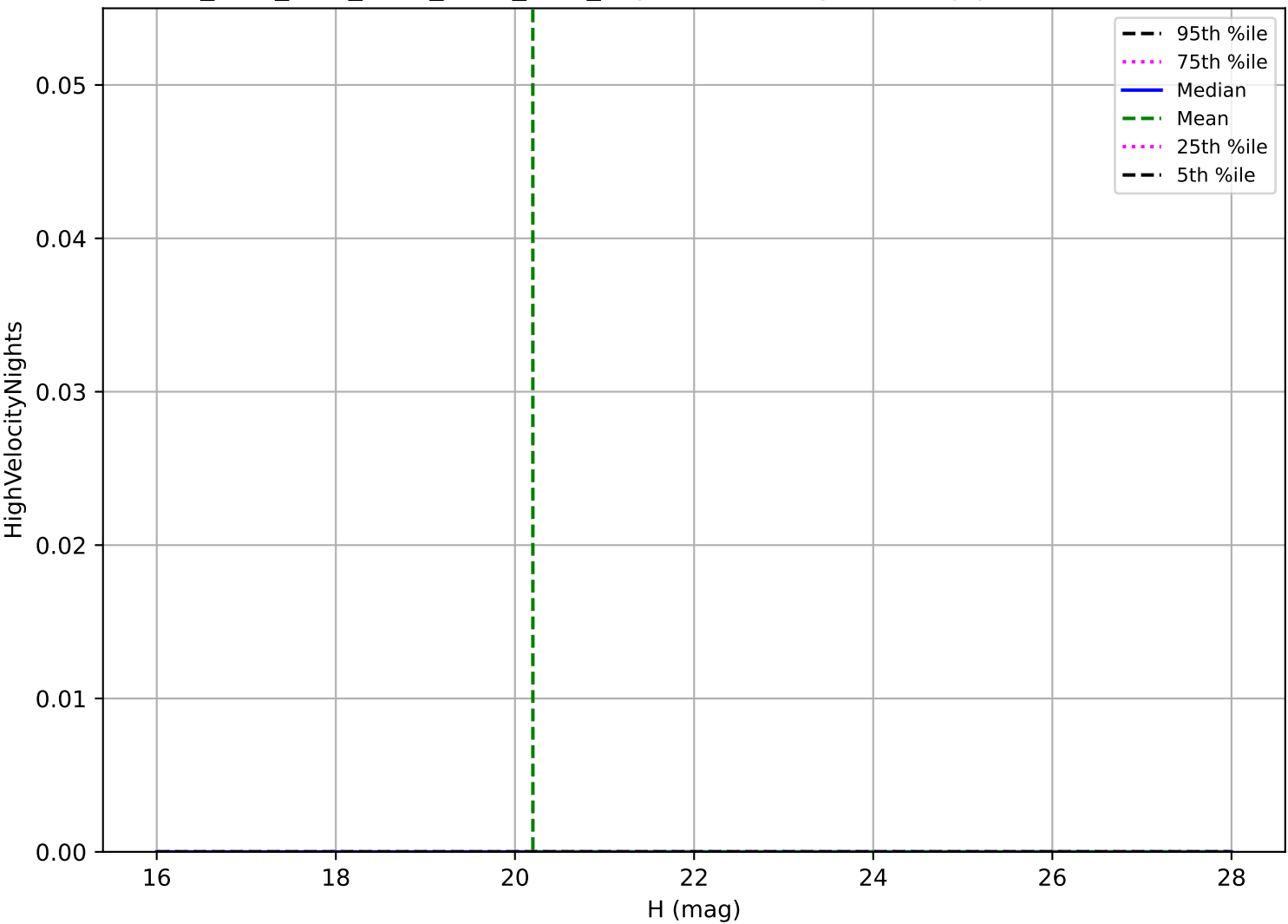
ddf_acor_sf10_lsf30_lsr50_v3.4_10yrs: Vatira High velocity pair detection loss
