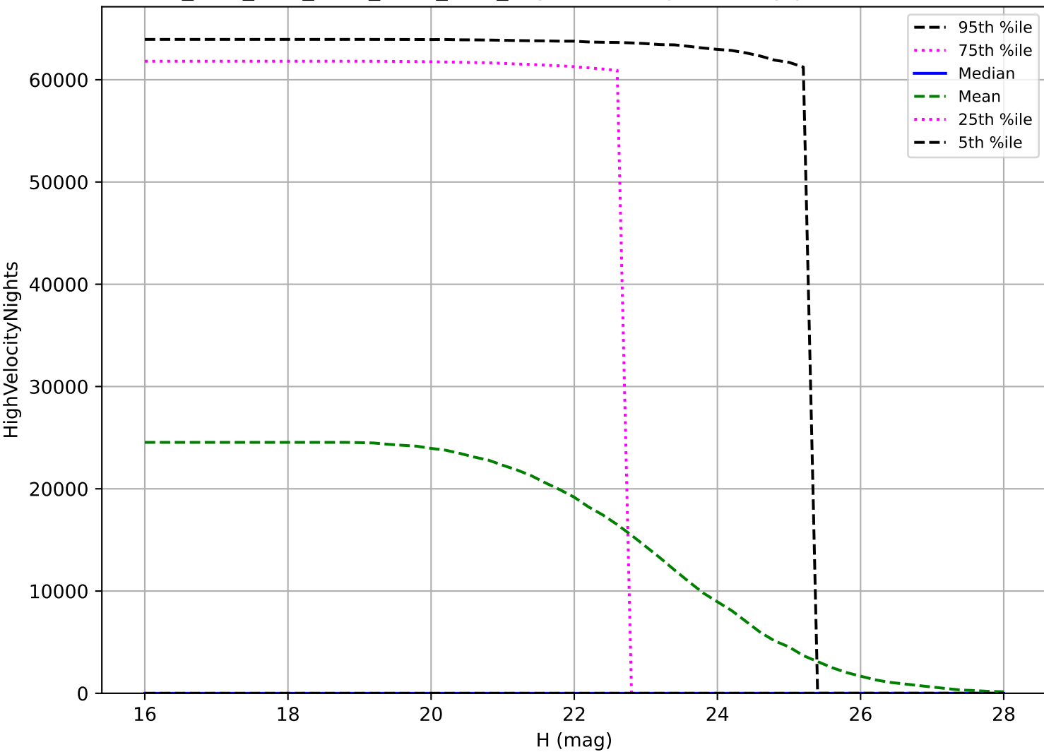
ddf_acor_sf10_lsf30_lsr50_v3.4_10yrs: PHA High velocity pair detection loss
