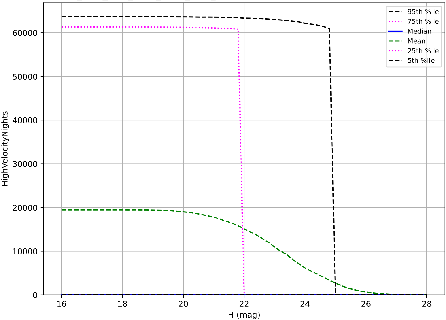
ddf_acor_sf10_lsf30_lsr50_v3.4_10yrs: NEO High velocity pair detection loss
