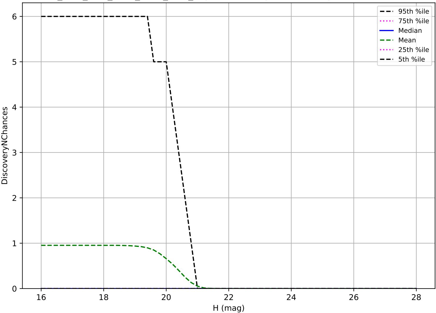
ddf_acor_sf10_lsf30_lsr50_v3.4_10yrs: Vatira 3 pairs in 15 nights detection loss
