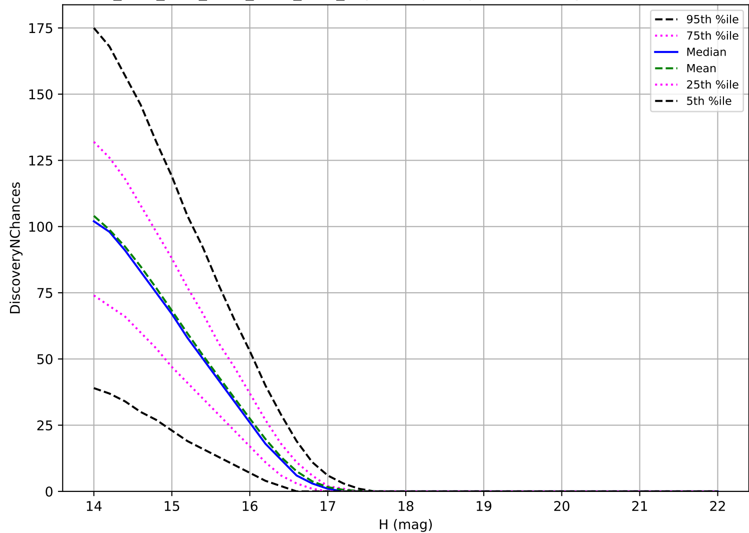
ddf_acor_sf10_lsf30_lsr50_v3.4_10yrs: Trojan 3 pairs in 15 nights detection loss
