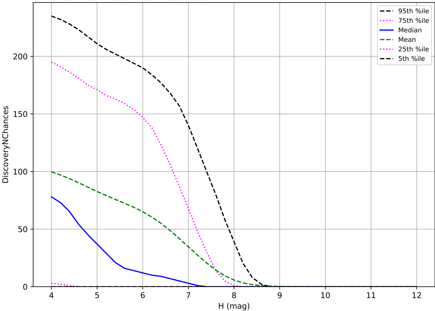
ddf_acor_sf10_lsf30_lsr50_v3.4_10yrs: TNO 3 pairs in 15 nights detection loss
