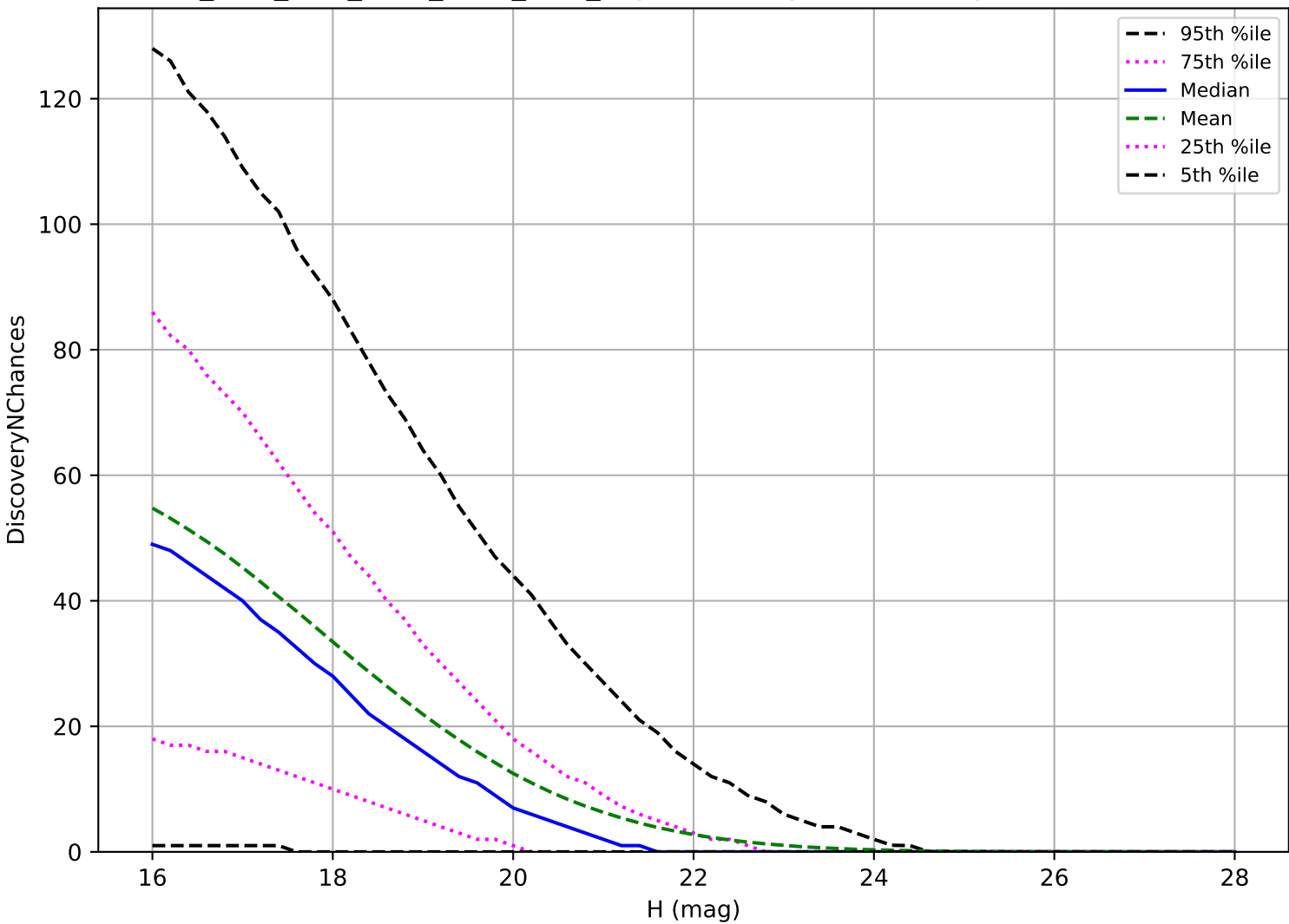
ddf_acor_sf10_lsf30_lsr50_v3.4_10yrs: PHA 3 pairs in 15 nights detection loss
