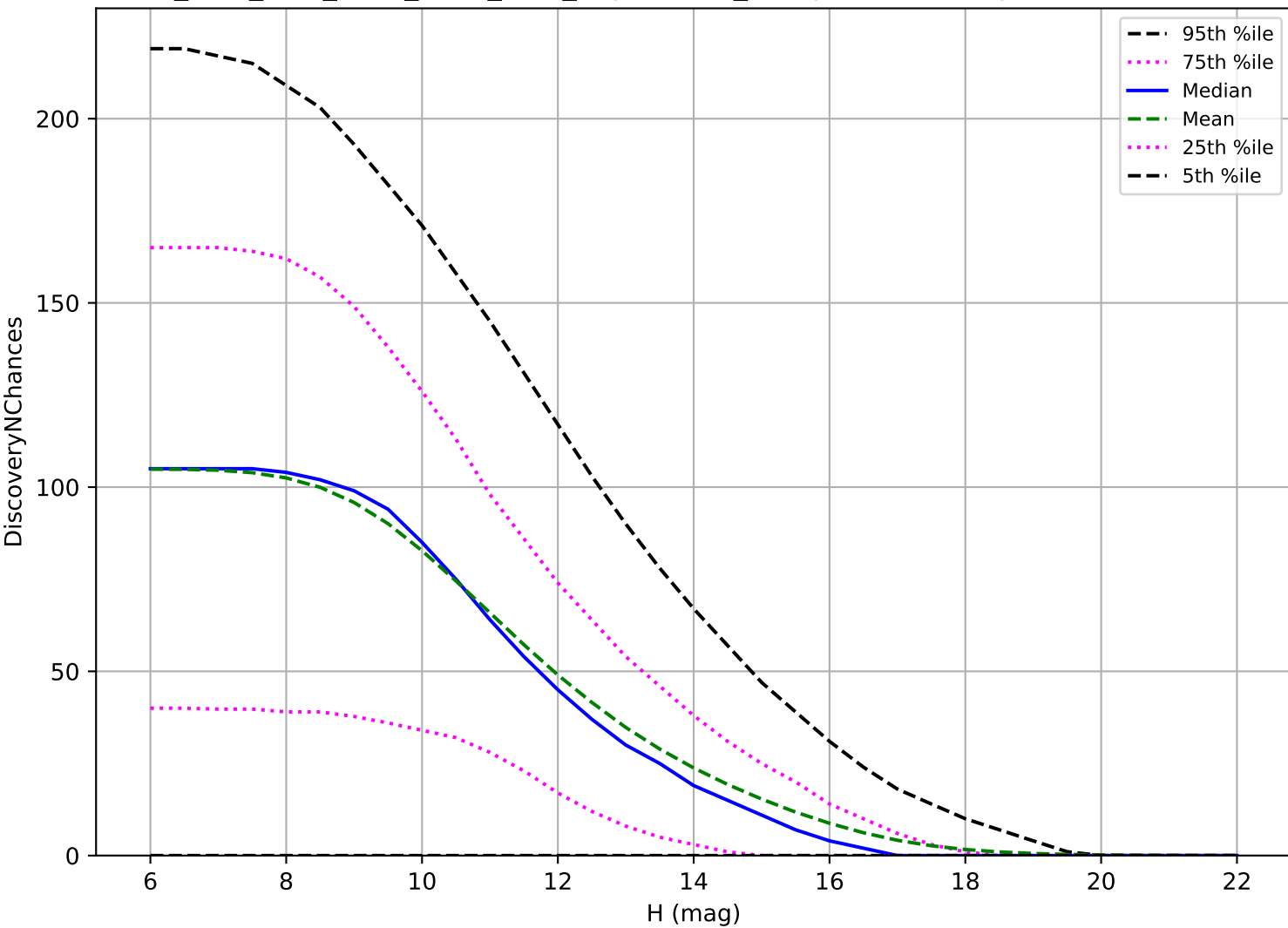
ddf_acor_sf10_lsf30_lsr50_v3.4_10yrs: OCC_r5 3 pairs in 15 nights detection loss
