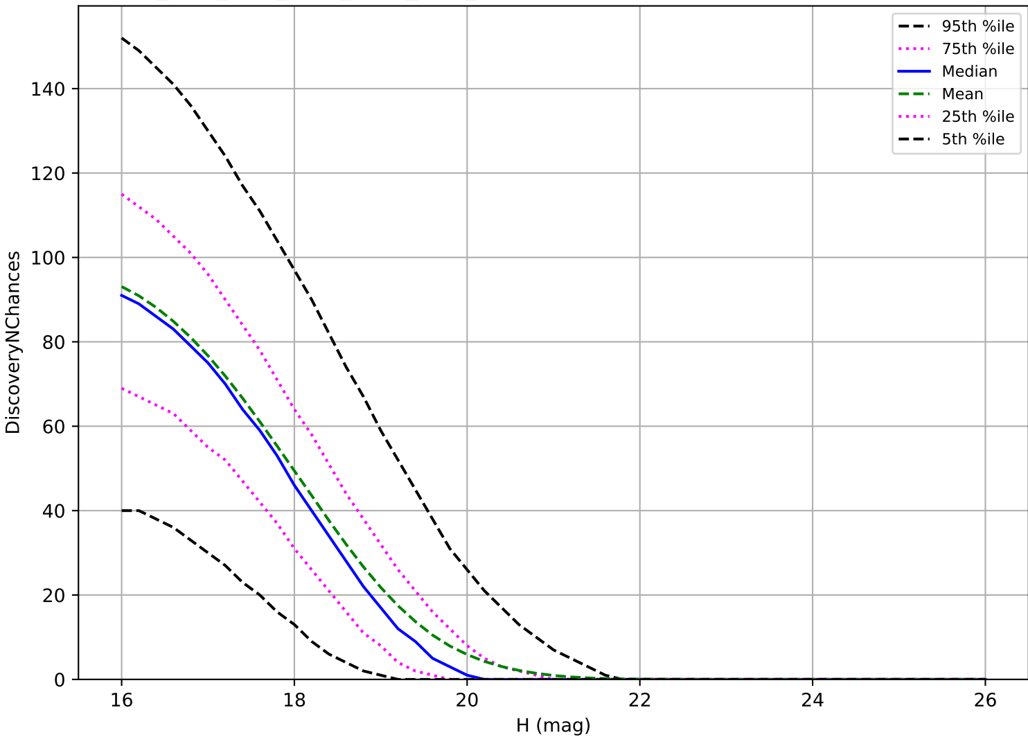
ddf_acor_sf10_lsf30_lsr50_v3.4_10yrs: MBA 3 pairs in 15 nights detection loss
