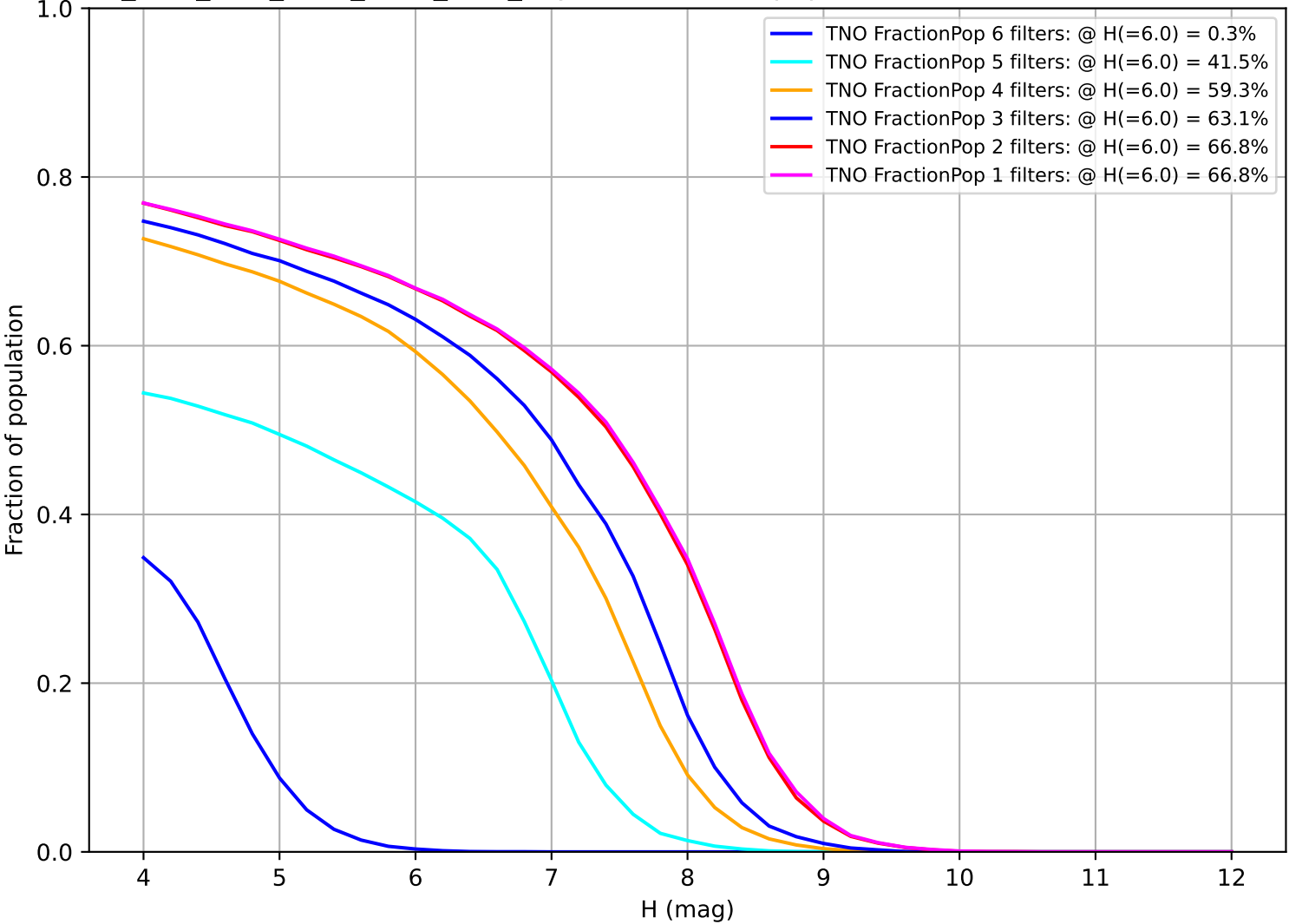
ddf_acor_sf10_lsf30_lsr50_v3.4_10yrs: Fraction of population with colors in X filters TNO
