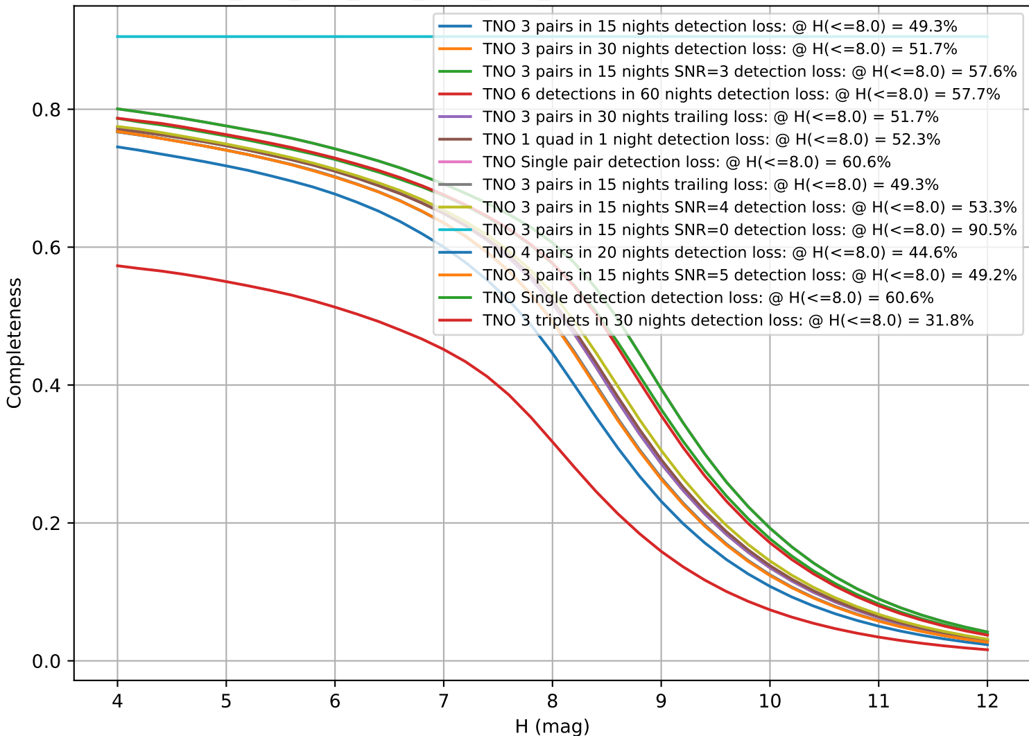
ddf_acor_sf10_lsf30_lsr50_v3.4_10yrs: CumulativeCompleteness
