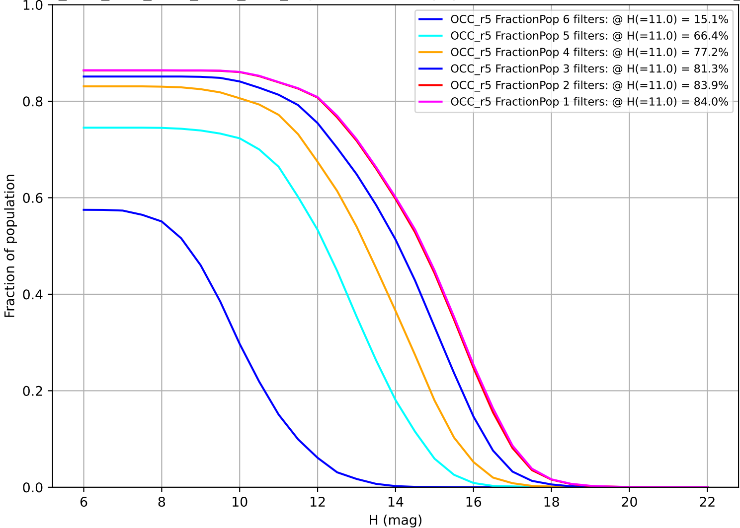
ddf_acor_sf10_lsf30_lsr50_v3.4_10yrs: Fraction of population with colors in X filters OCC_r5
