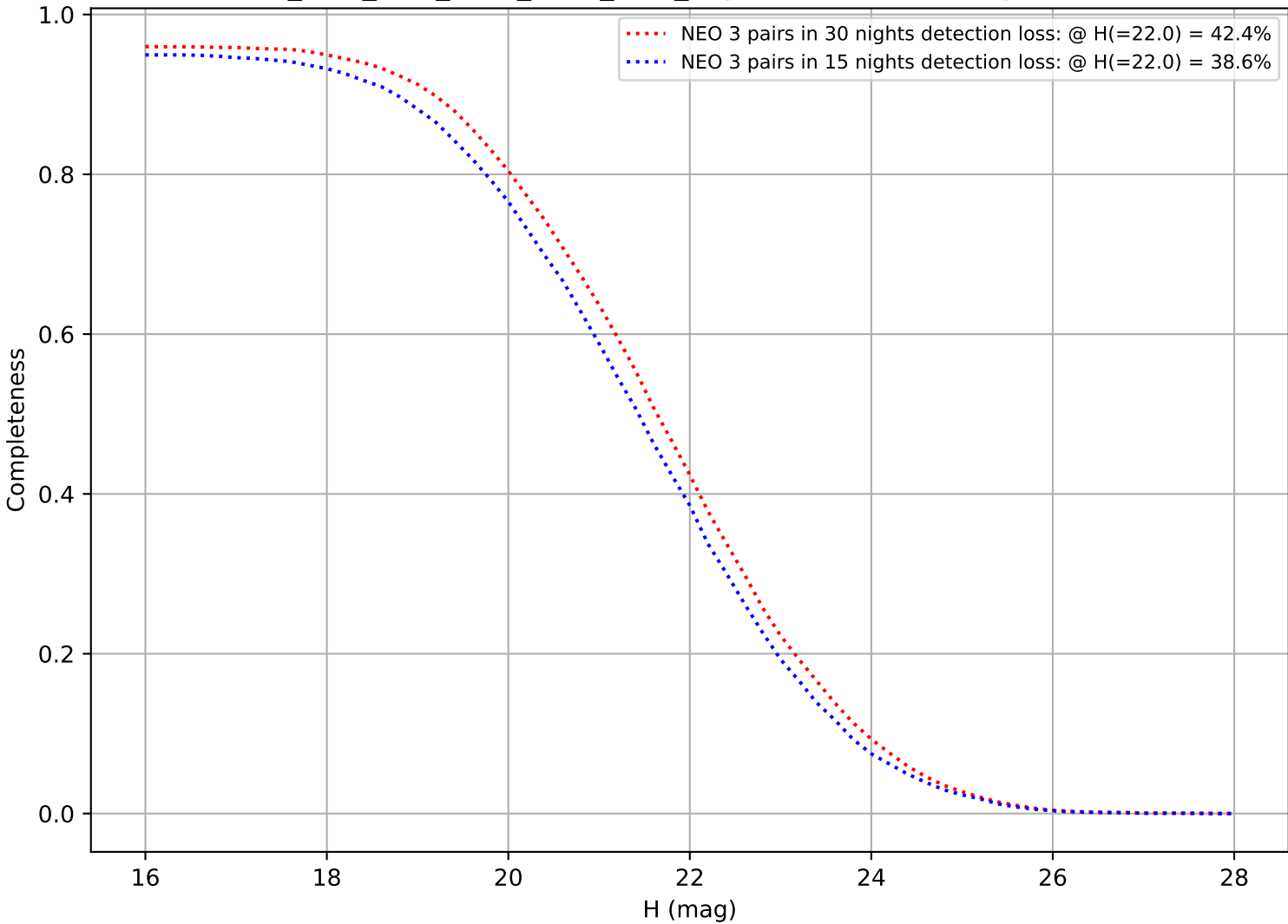
ddf_acor_sf10_lsf30_lsr50_v3.4_10yrs: DifferentialCompleteness
