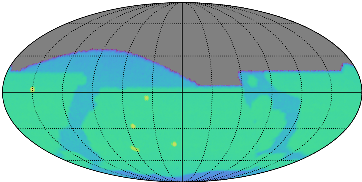
ddf_acor_sf10_lsf30_lsr50_v3.4_10yrs i: SurfaceBrightLimit
