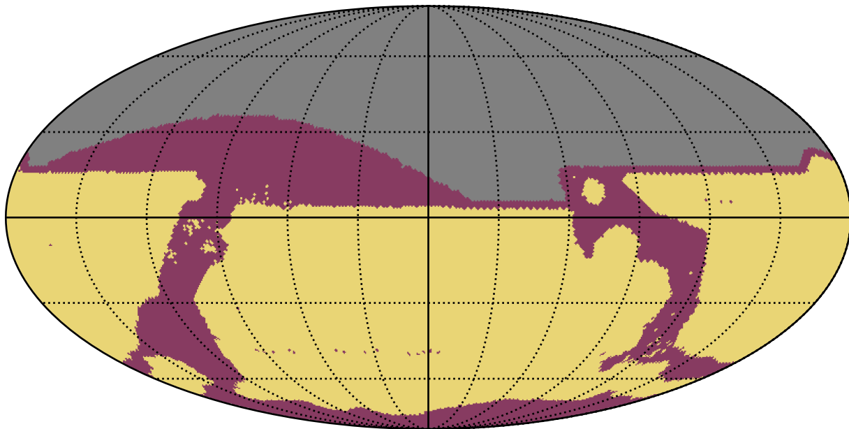
ddf_acor_sf10_lsf30_lsr50_v3.4_10yrs : RapidRevisits
