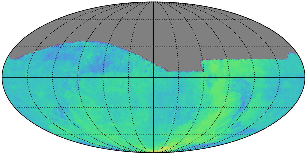
ddf_acor_sf10_lsf30_lsr50_v3.4_10yrs : Parallax Coverage @ 24.0
