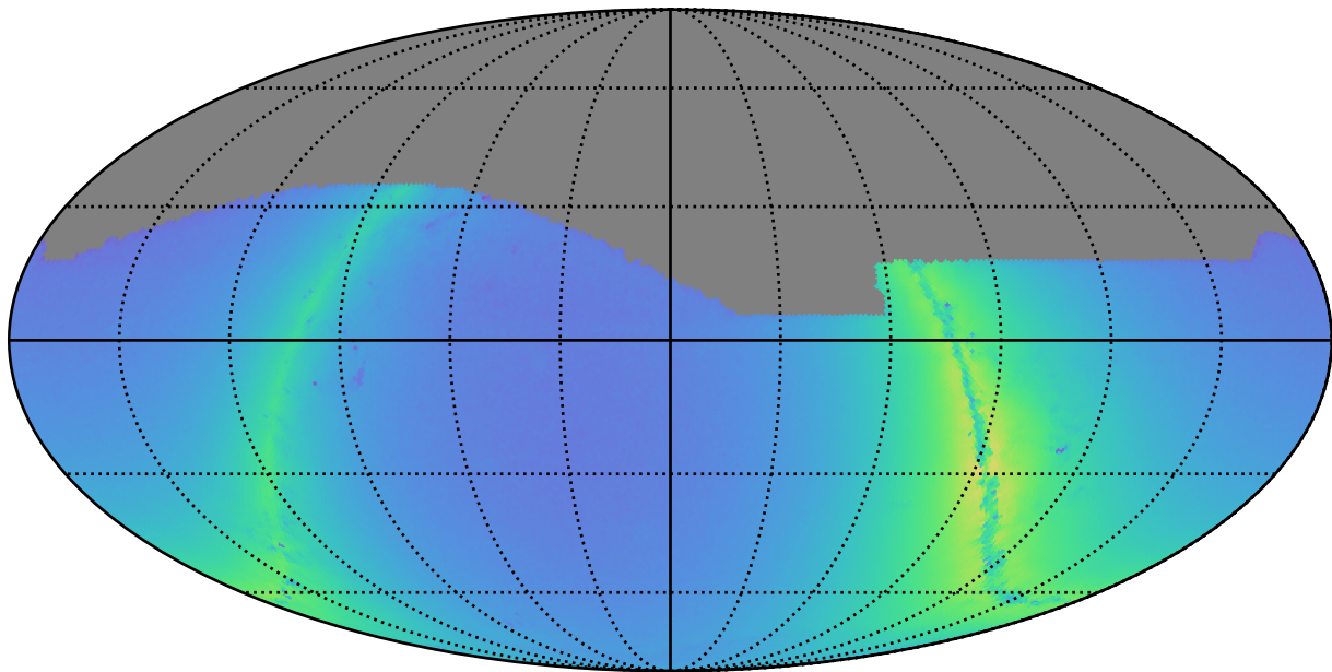
ddf_acor_sf10_lsf30_lsr50_v3.4_10yrs r: Nstars_no_crowding
