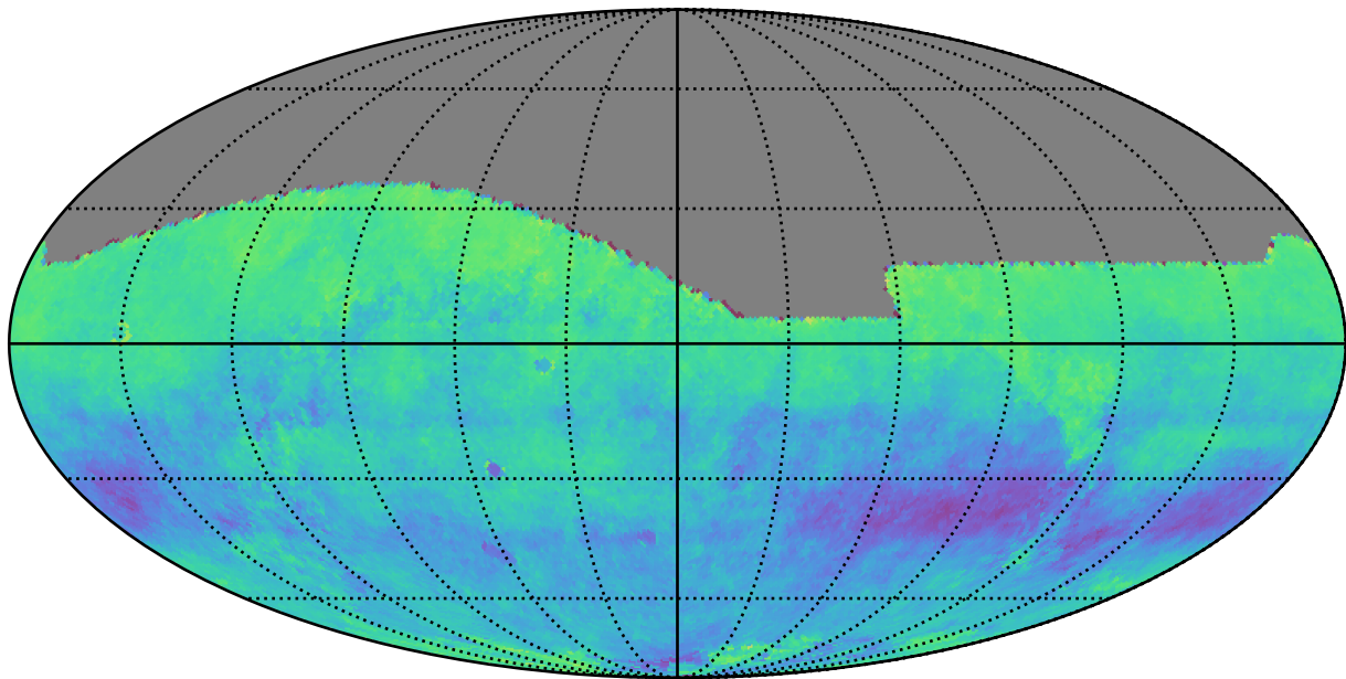
ddf_acor_sf10_lsf30_lsr50_v3.4_10yrs r: Kuiper rotSkyPos
