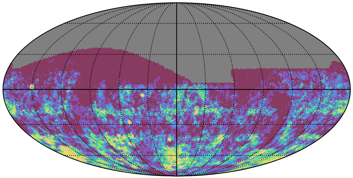
ddf_acor_sf10_lsf30_lsr50_v3.4_10yrs r band: Gaps_3hr
