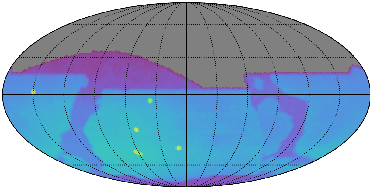
ddf_acor_sf10_lsf30_lsr50_v3.4_10yrs : Brown Dwarf, L7
