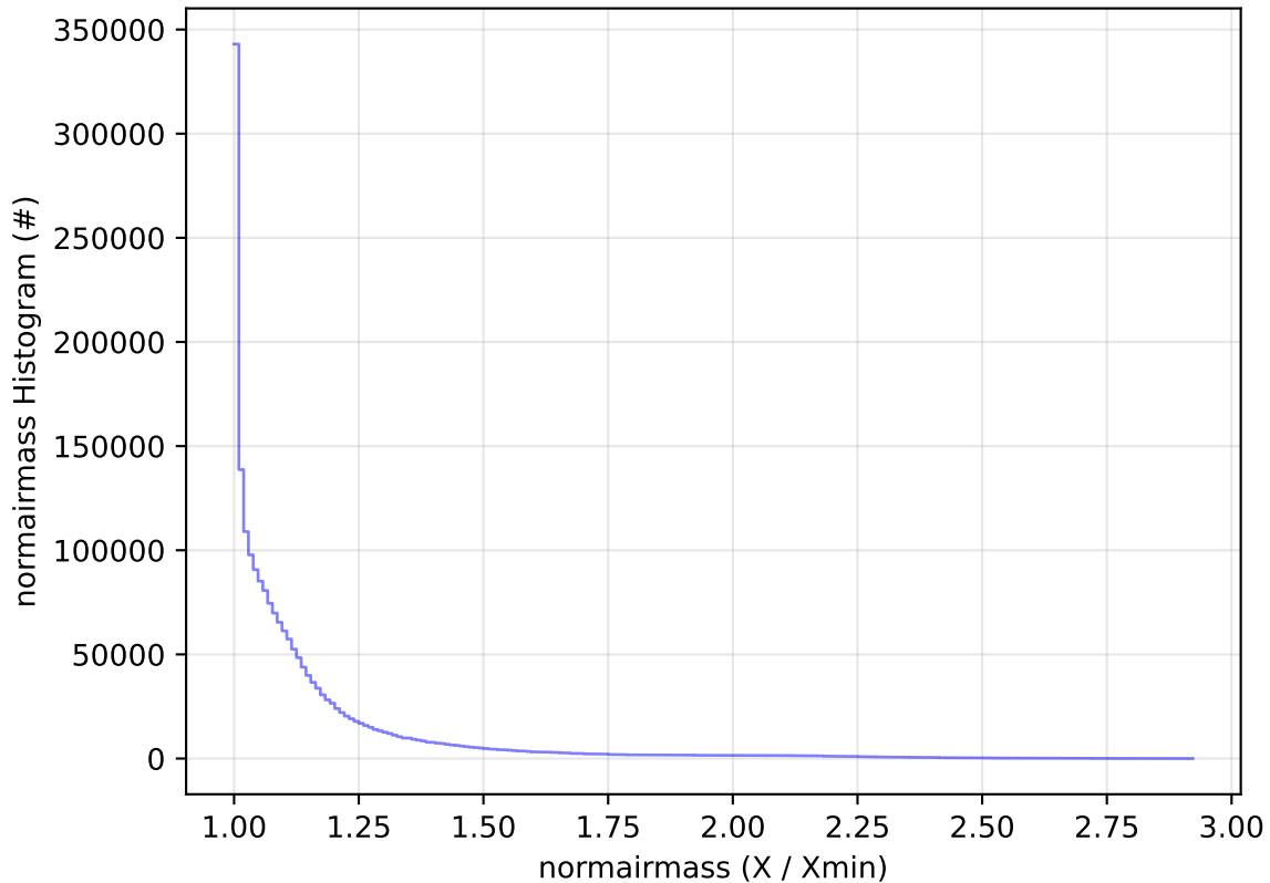
ddf_acor_sf10_lsf30_lsr50_v3.4_10yrs WFD all bands: normairmass Histogram
