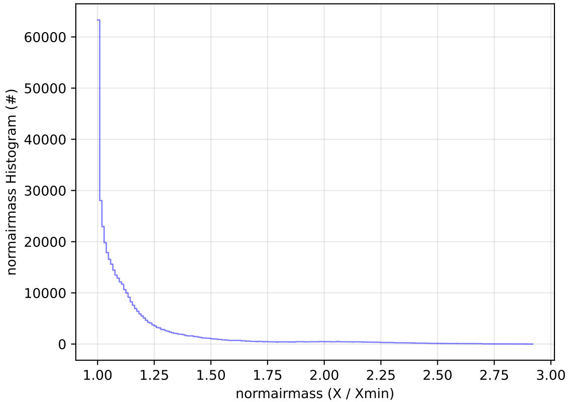
ddf_acor_sf10_lsf30_lsr50_v3.4_10yrs All sky z band: normairmass Histogram
