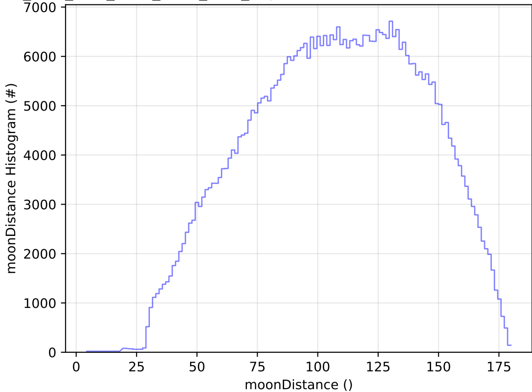
ddf_acor_sf10_lsf30_lsr50_v3.4_10yrs WFD r band: moonDistance Histogram
