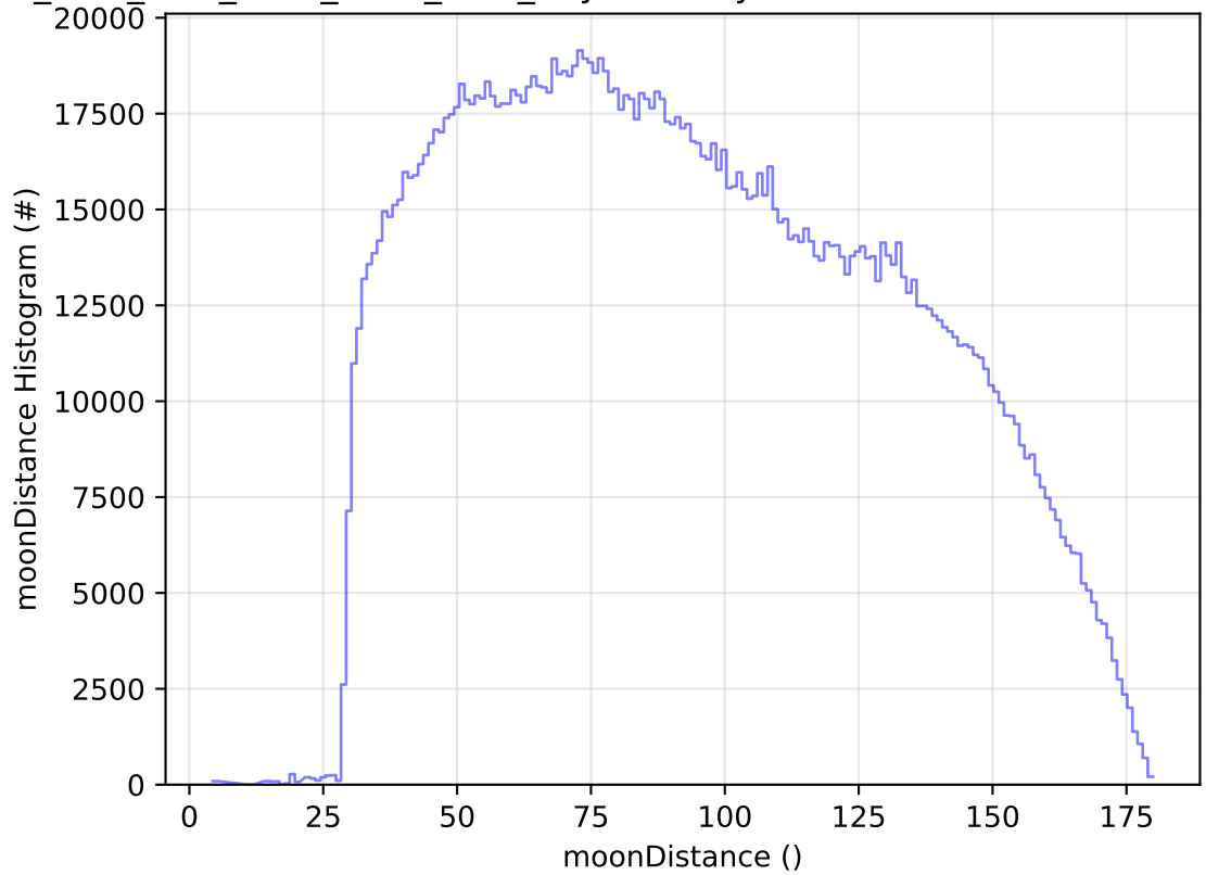
ddf_acor_sf10_lsf30_lsr50_v3.4_10yrs All sky all bands: moonDistance Histogram
