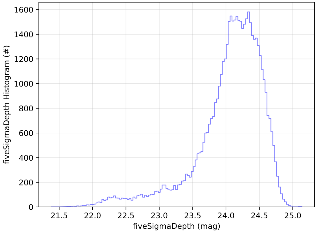
ddf_acor_sf10_lsf30_lsr50_v3.4_10yrs Yr 1 r band: fiveSigmaDepth Histogram
