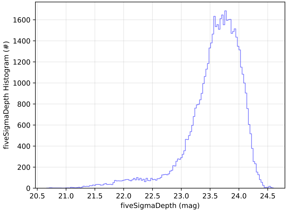
ddf_acor_sf10_lsf30_lsr50_v3.4_10yrs Yr 1 i band: fiveSigmaDepth Histogram
