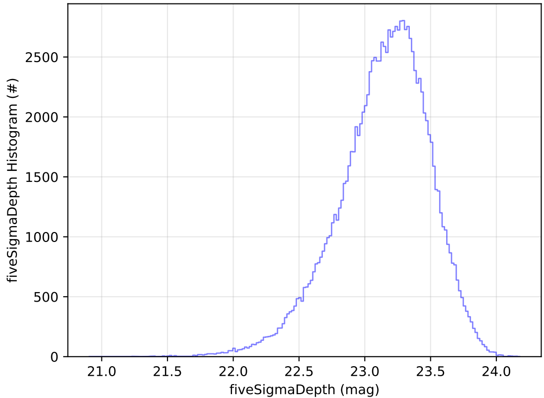
ddf_acor_sf10_lsf30_lsr50_v3.4_10yrs WFD u band: fiveSigmaDepth Histogram
